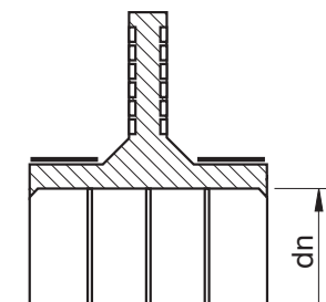
dn=90 ÷ 315 mm
